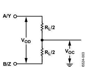
Figure 7. Differential Output Voltage and Common-Mode Voltage Drivers
